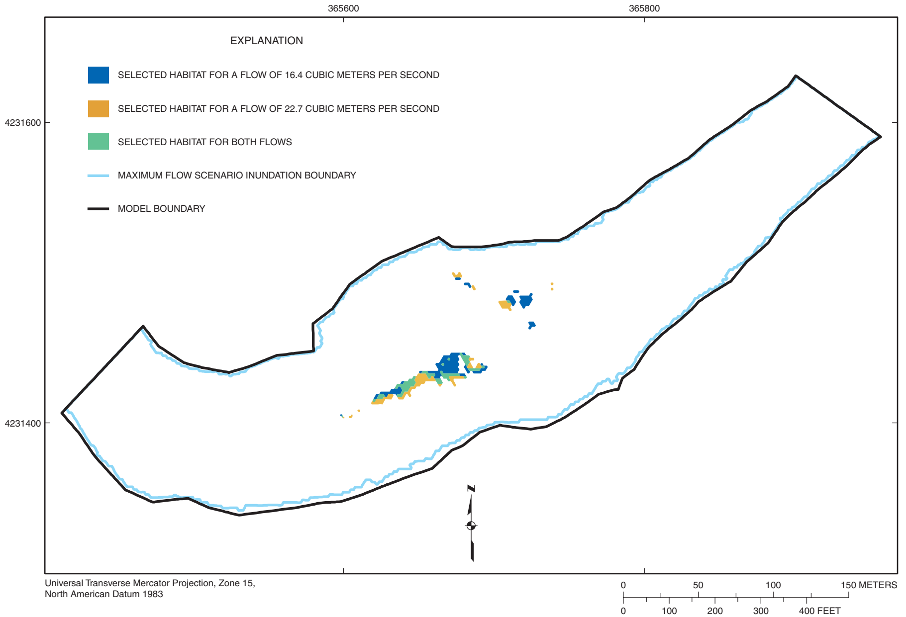
Figure 4-73. Selected habitat area distribution for habitat category 19 (stonecat) at flows of 16.4 and 22.7 cubic meters per second at Marais des Cygnes River site MDC2.
